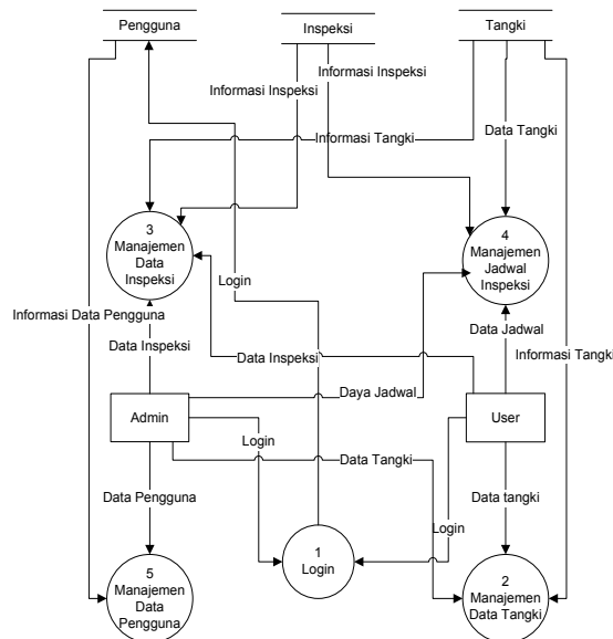
Gambar 3.5 Data Flow Diagram (DFD) Level 1
