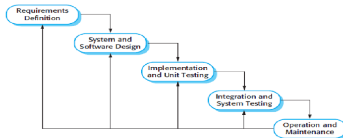
Gambar 1 Model Pengembangan Waterfall
