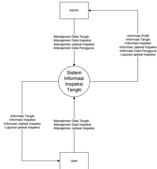
Gambar 3.3 Context Diagram
