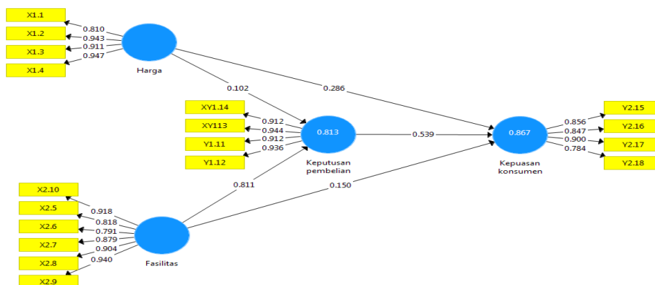
Gambar 2. Diagram SEM hasil proses bootstrapping
