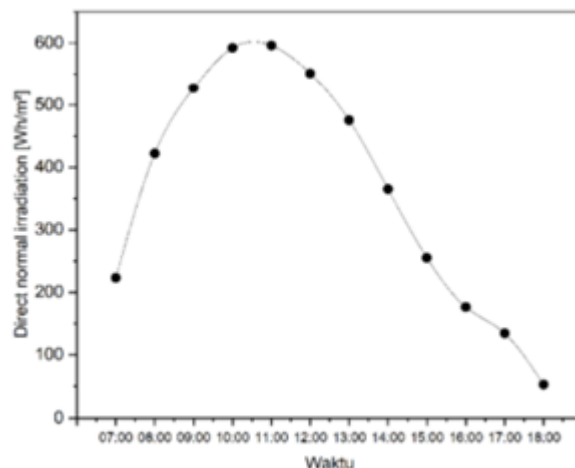
Gambar 1. Intensitas Radiasi Matahari (W/m 2 )
