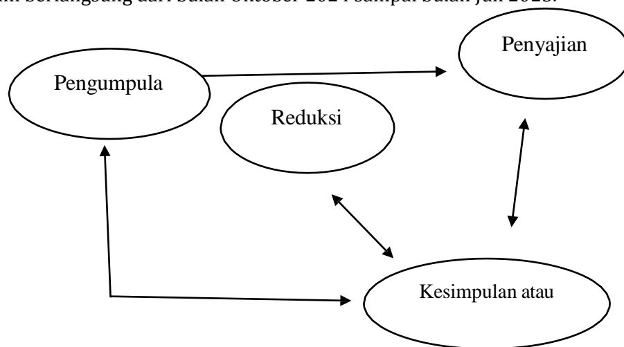
Gambar 1 Model Analisis Interaktif Miles & Huberman
