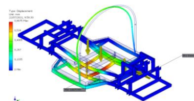
Gambar 12. Hasil Displacement
